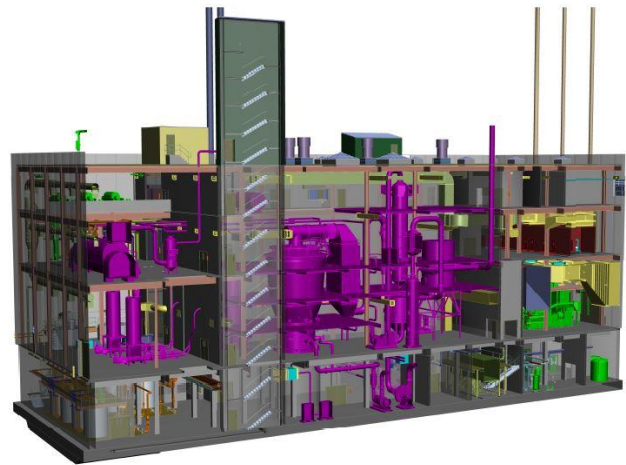
3D rendering of new solids handling building
